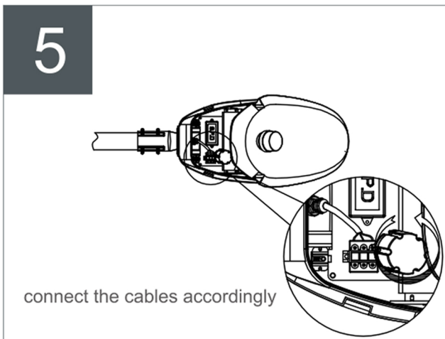
Fixed Mounting
